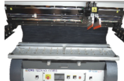
Double sided PCB pin clamping with support
