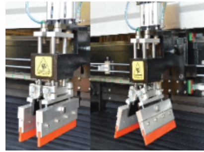
Adjustable squeegee angle upto 30°
