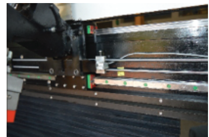
Double Linear Guide for Squeegee Movement
